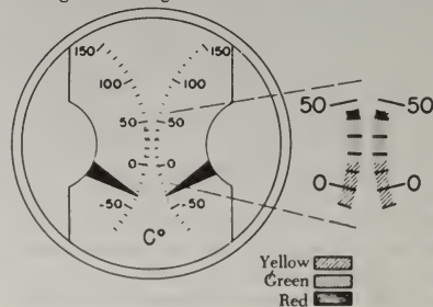
FIGURE 10-23. Carburetor air temperature gage.
